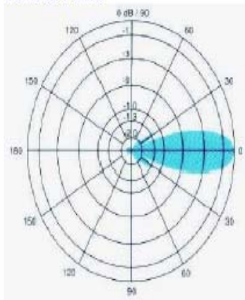
Vertical Plane
