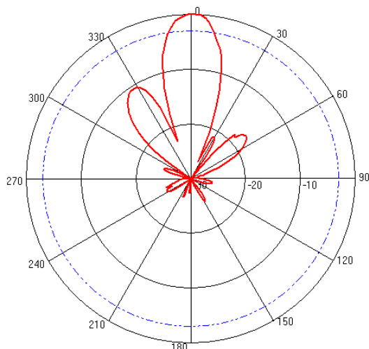
Vertical Pattern
