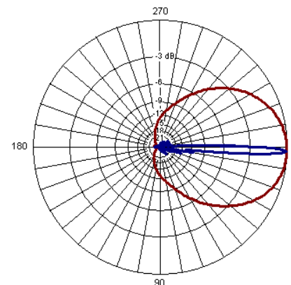
2 DEGREE DOWN TILT PLOT
